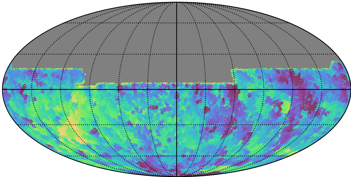
too_100_1v3.4_10yrs All sky y band: Min fiveSigmaDepth
