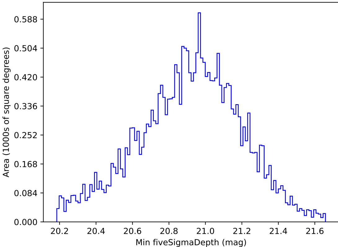
too_100_1v3.4_10yrs All sky y band: Min fiveSigmaDepth
