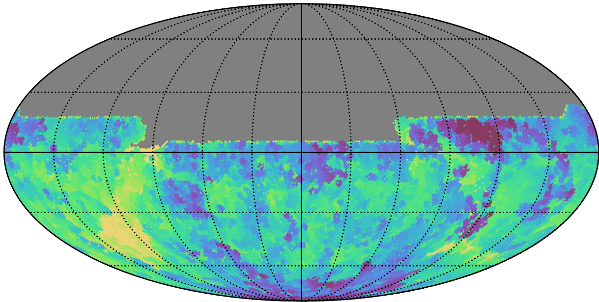
too_100_1v3.4_10yrs All sky u band: Min fiveSigmaDepth
