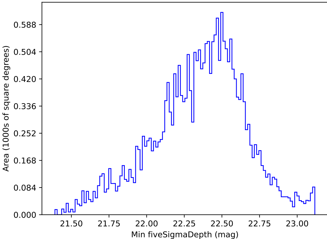
too_100_1v3.4_10yrs All sky u band: Min fiveSigmaDepth
