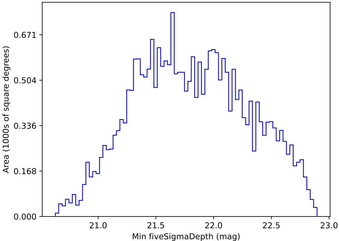
too_100_1v3.4_10yrs All sky i band: Min fiveSigmaDepth
