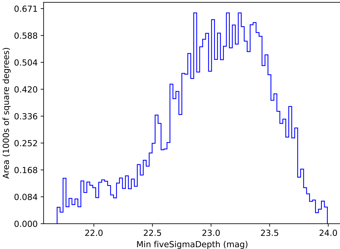
too_100_1v3.4_10yrs All sky g band: Min fiveSigmaDepth
