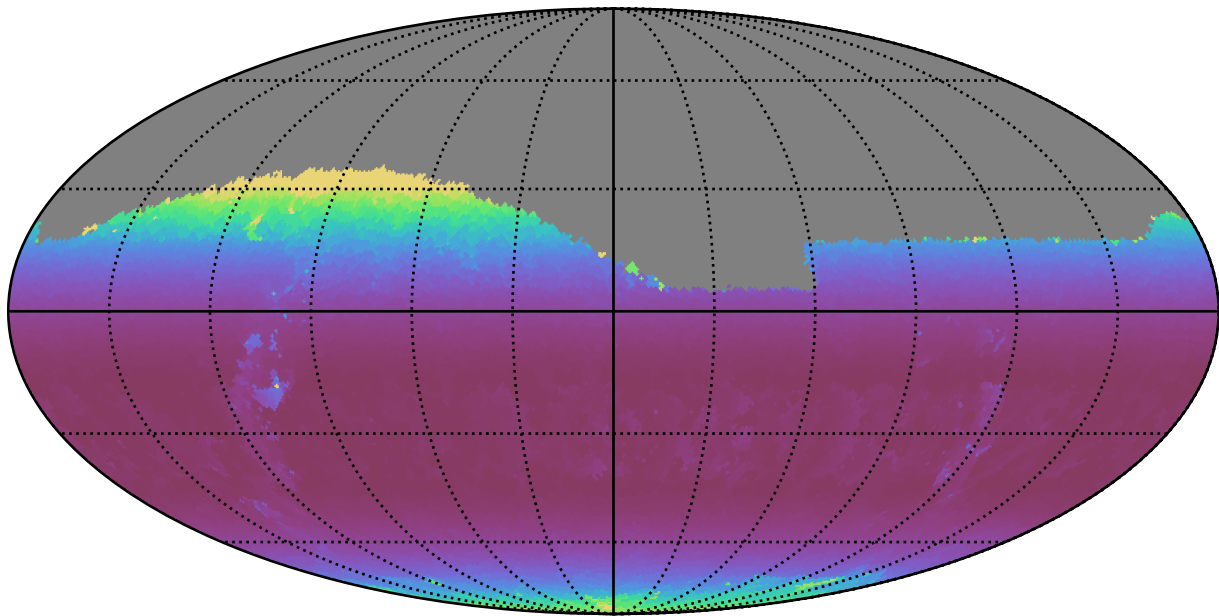
too_100_1v3.4_10yrs Yr 1 z band: Min airmass
