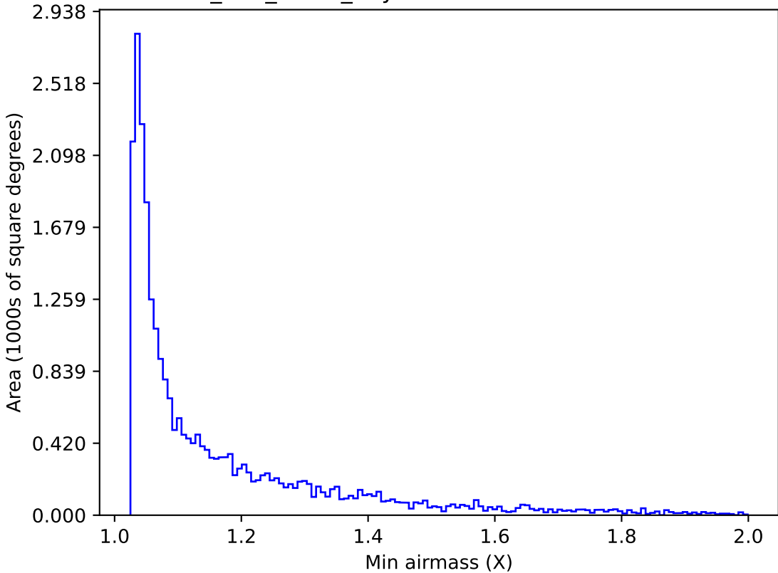
too_100_1v3.4_10yrs Yr 1 z band: Min airmass
