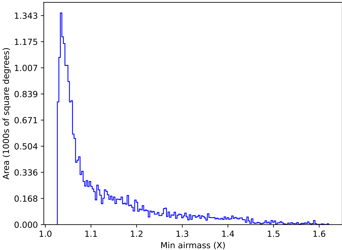
too_100_1v3.4_10yrs Yr 1 y band: Min airmass
