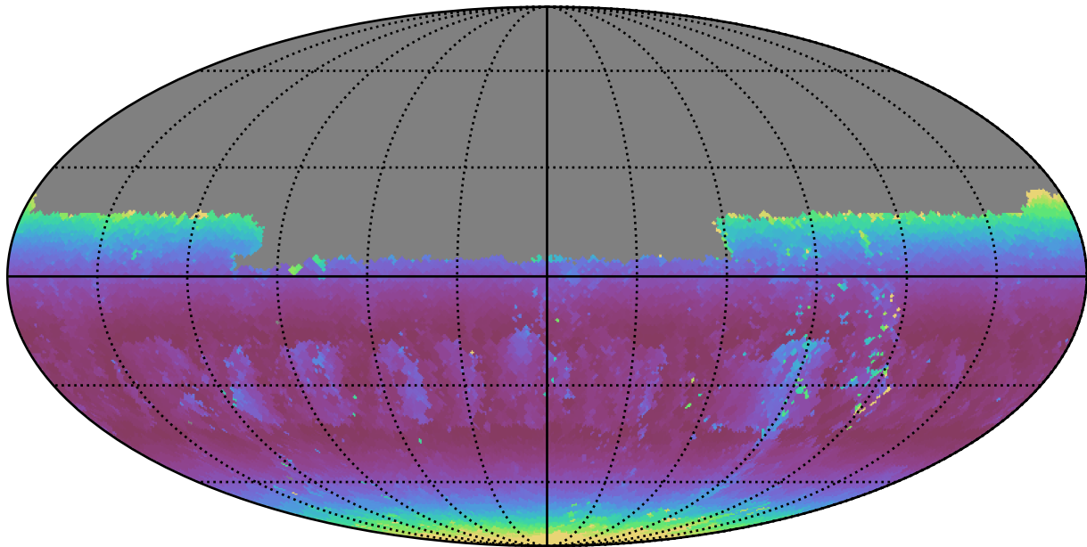
too_100_1v3.4_10yrs Yr 1 u band: Min airmass
