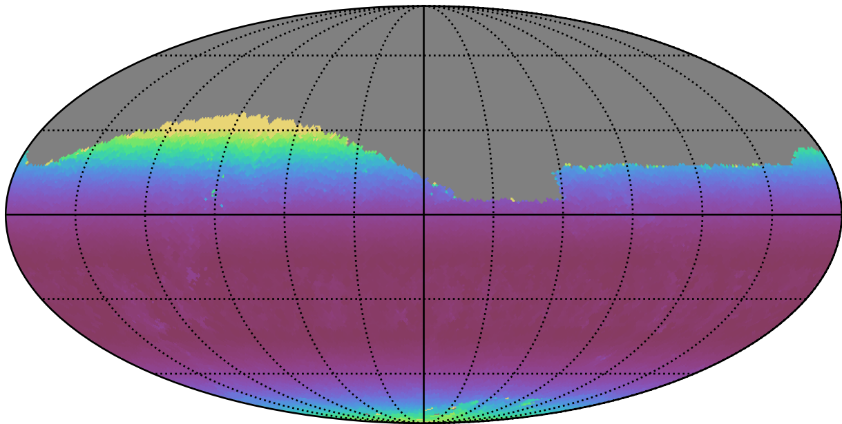
too_100_1v3.4_10yrs Yr 1 r band: Min airmass
