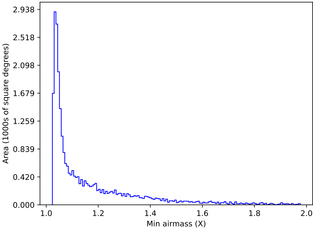
too_100_1v3.4_10yrs Yr 1 r band: Min airmass
