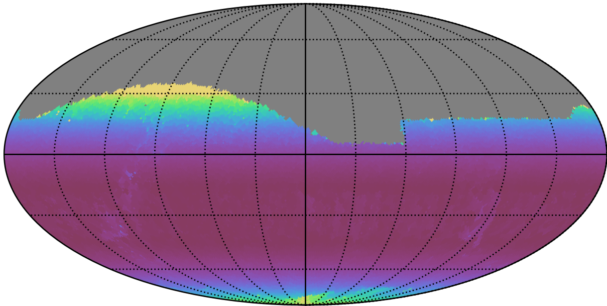
too_100_1v3.4_10yrs Yr 1 i band: Min airmass
