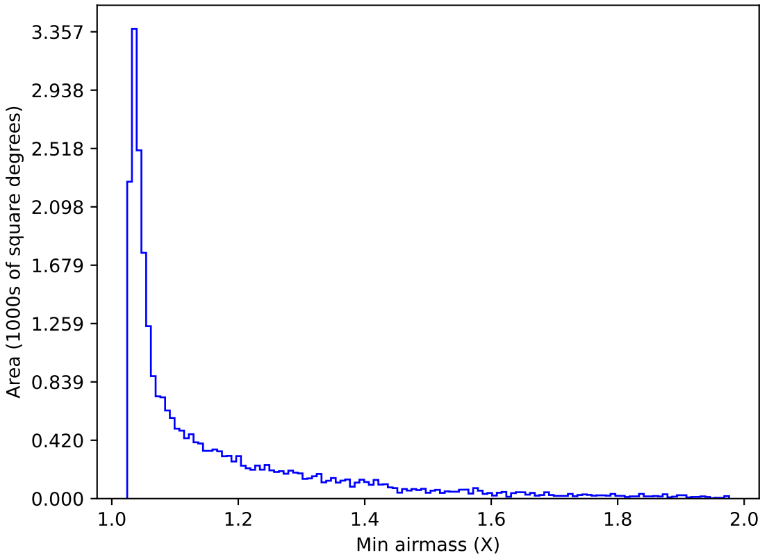
too_100_1v3.4_10yrs Yr 1 i band: Min airmass
