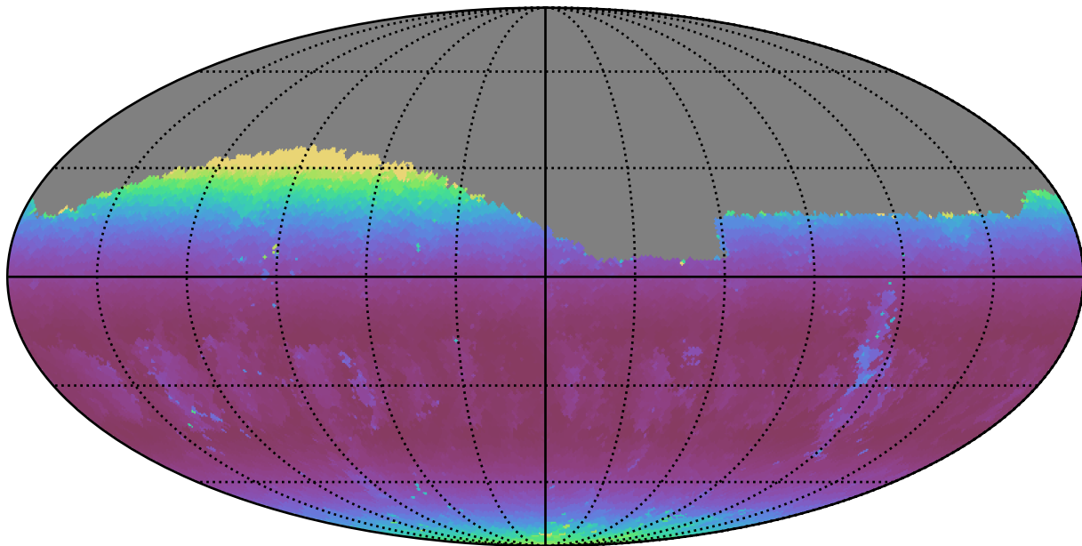
too_100_1v3.4_10yrs Yr 1 g band: Min airmass
