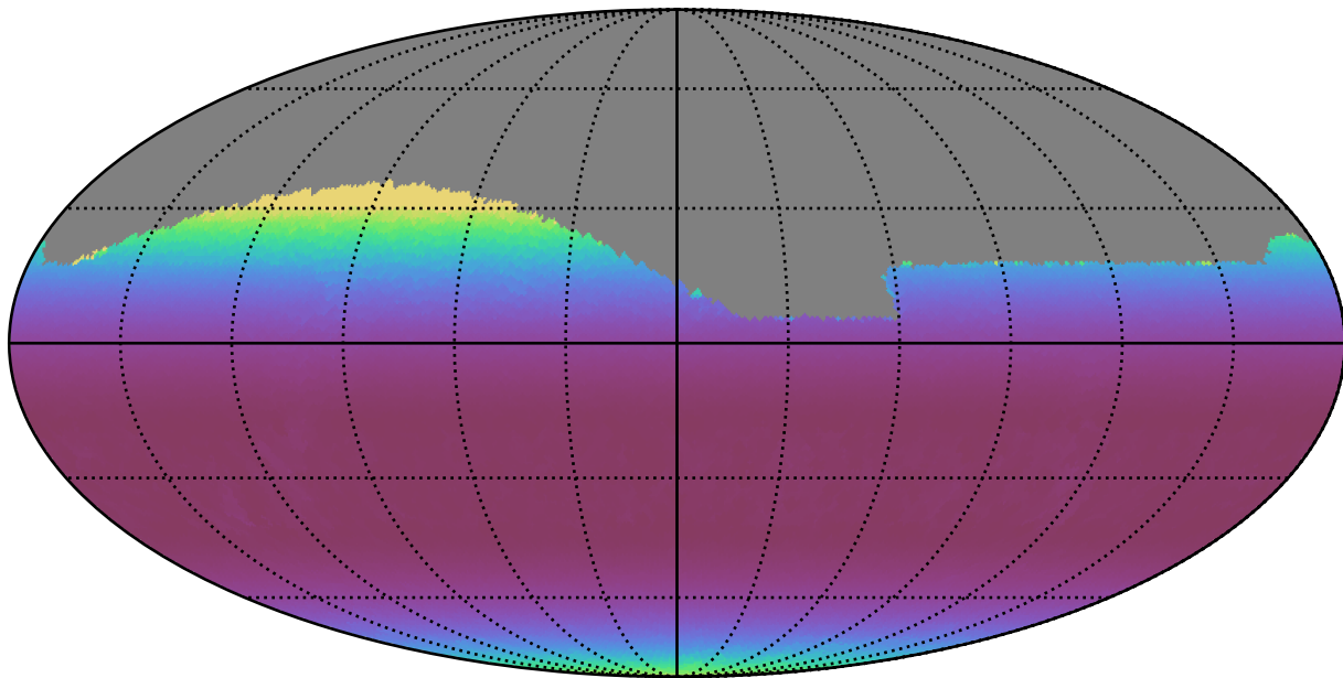
too_100_1v3.4_10yrs Yr 1 all bands: Min airmass
