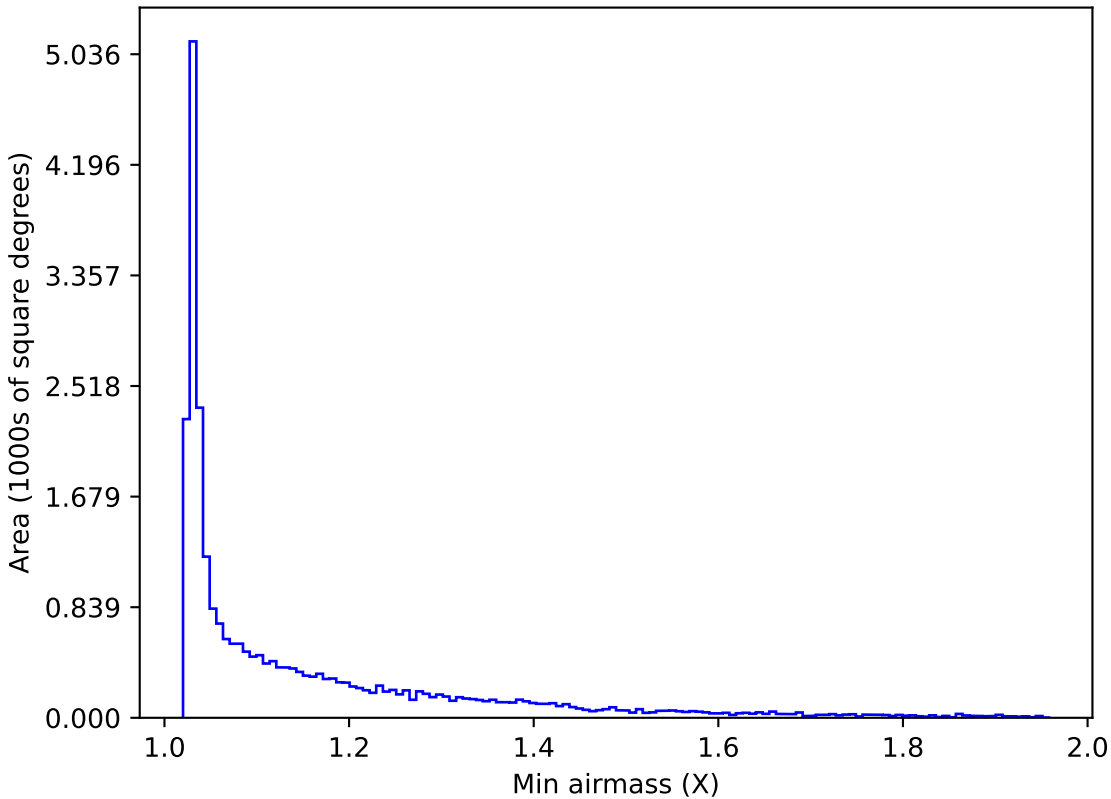
too_100_1v3.4_10yrs Yr 1 all bands: Min airmass
