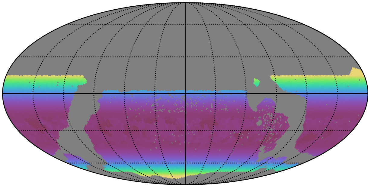
too_100_1v3.4_10yrs WFD z band: Min airmass
