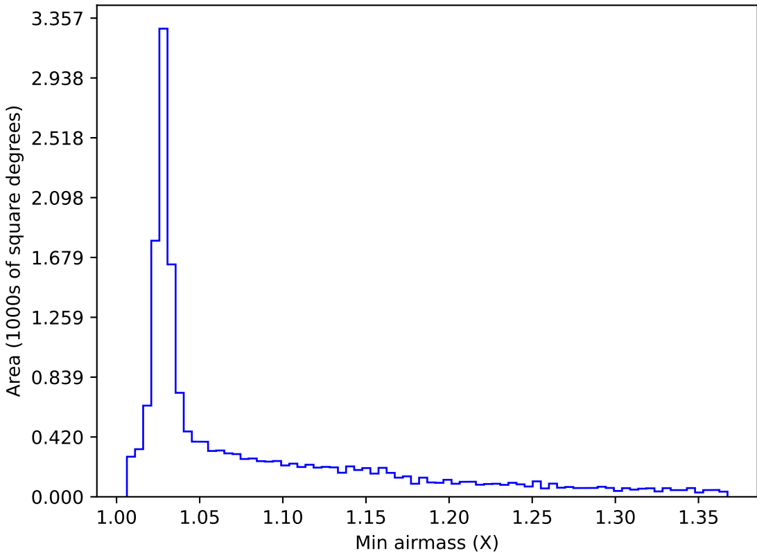
too_100_1v3.4_10yrs WFD z band: Min airmass
