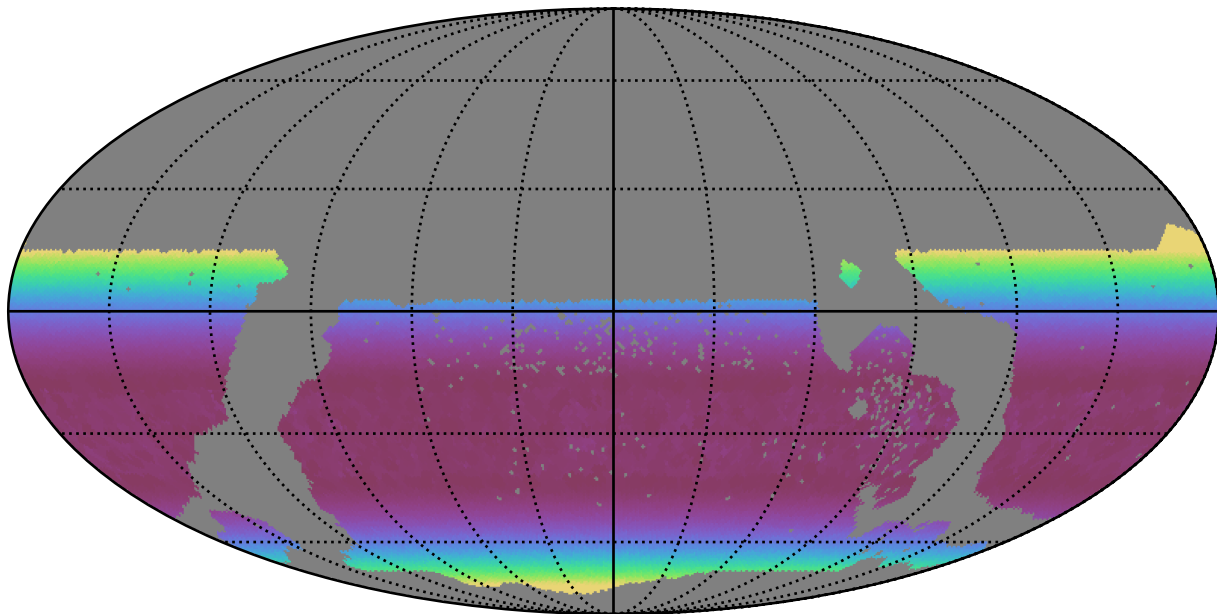
too_100_1v3.4_10yrs WFD y band: Min airmass
