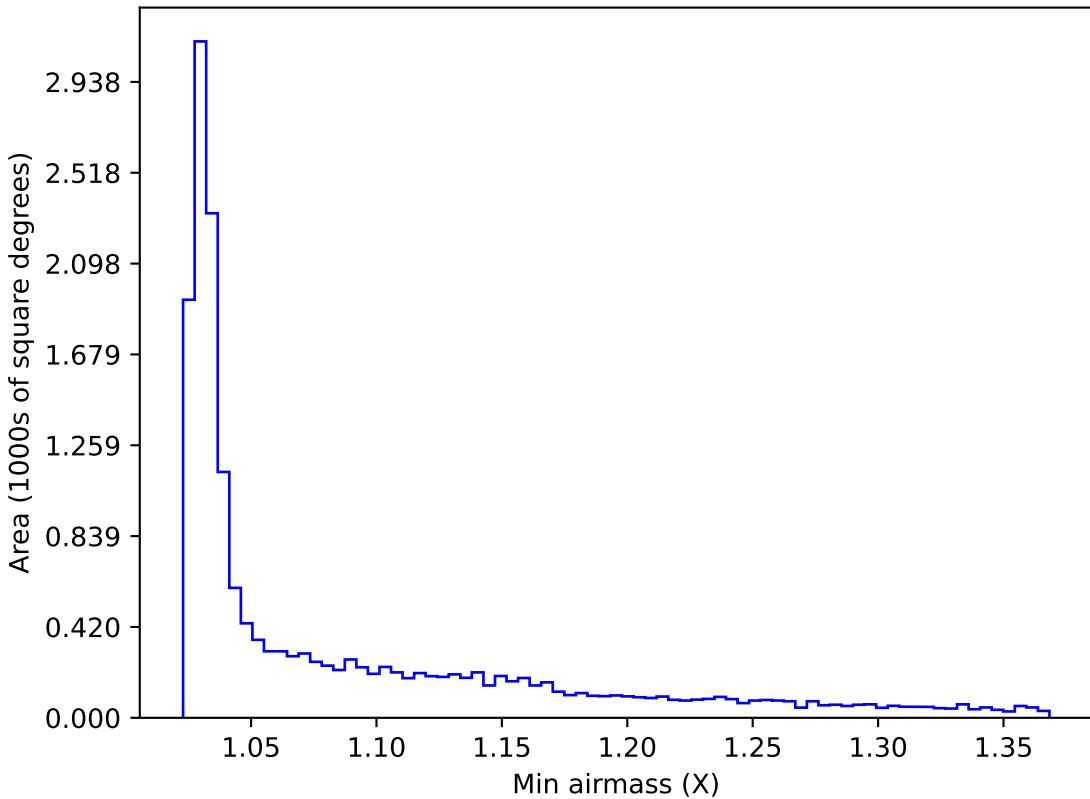
too_100_1v3.4_10yrs WFD y band: Min airmass
