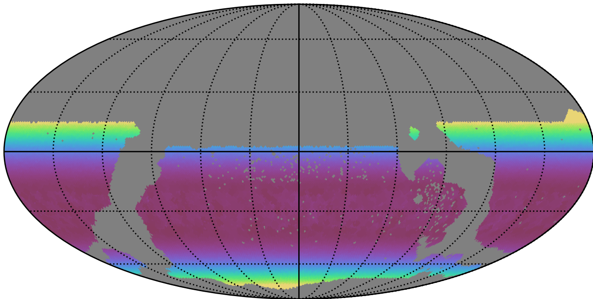
too_100_1v3.4_10yrs WFD r band: Min airmass
