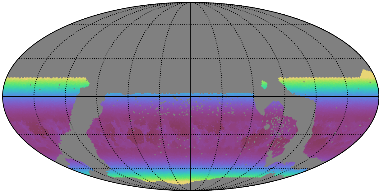
too_100_1v3.4_10yrs WFD g band: Min airmass
