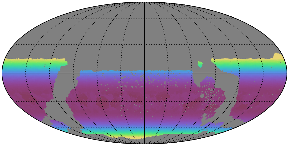
too_100_1v3.4_10yrs WFD all bands: Min airmass
