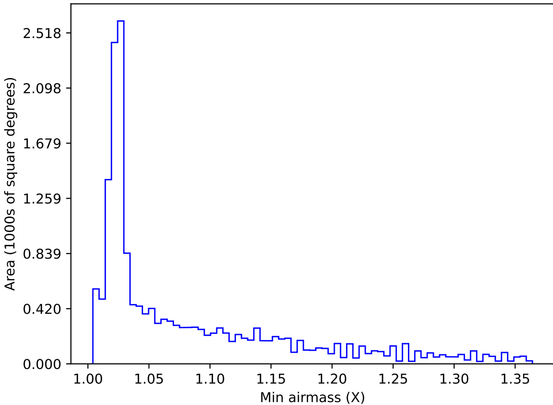
too_100_1v3.4_10yrs WFD all bands: Min airmass
