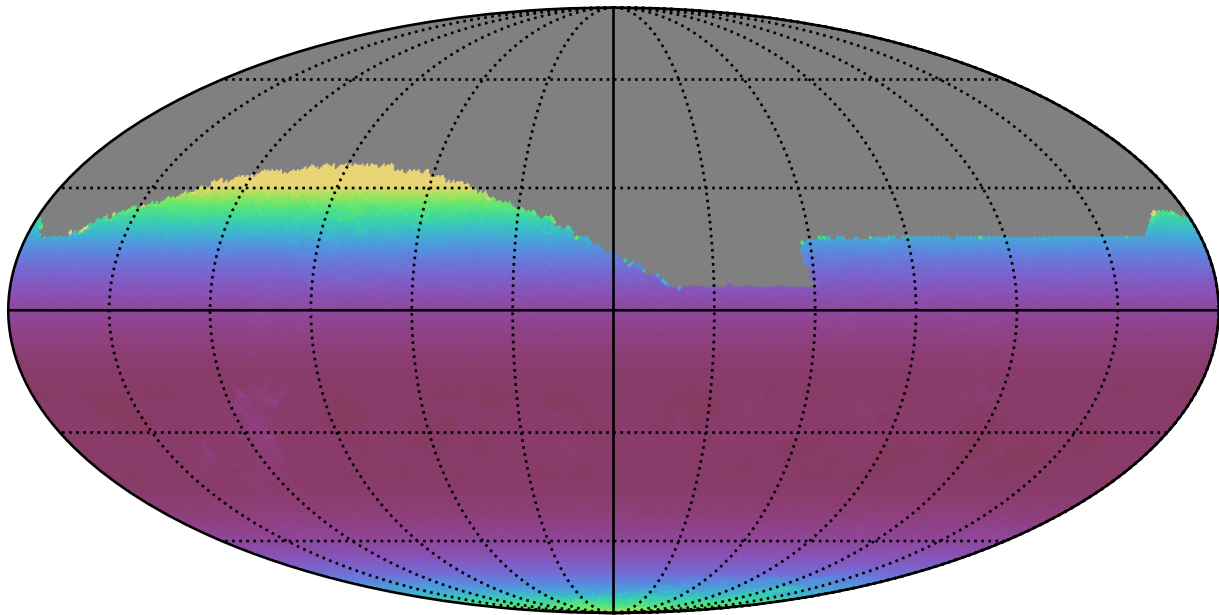
too_100_1v3.4_10yrs All sky z band: Min airmass
