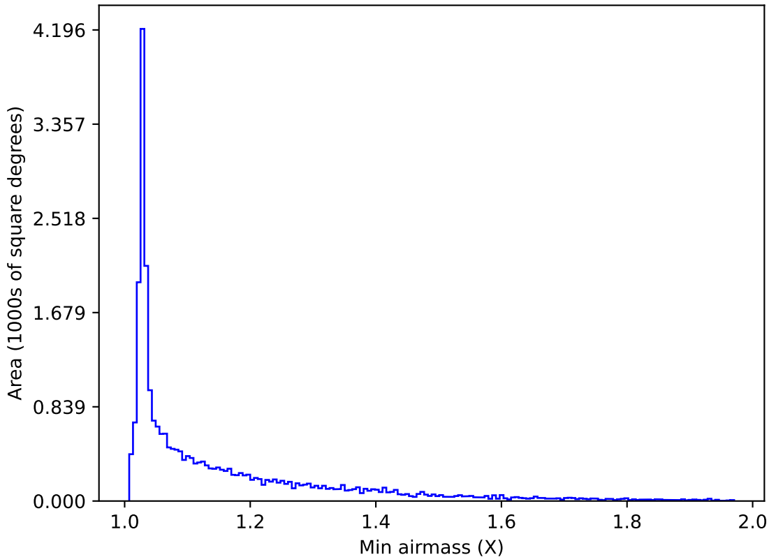
too_100_1v3.4_10yrs All sky z band: Min airmass
