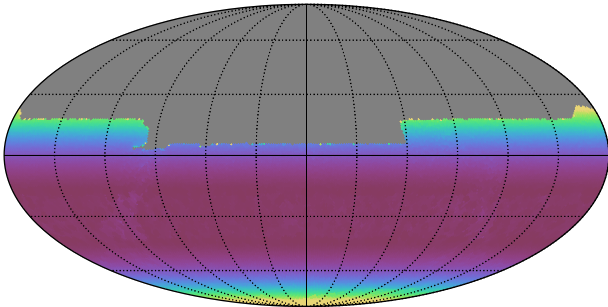
too_100_1v3.4_10yrs All sky y band: Min airmass
