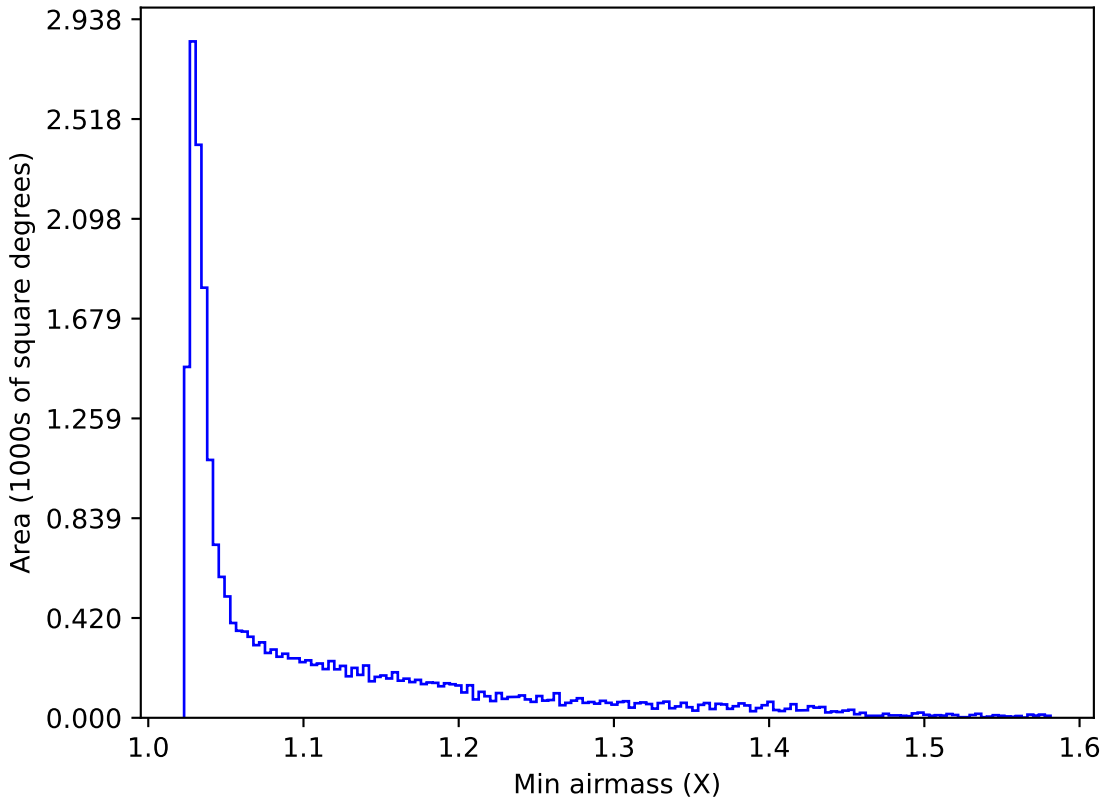
too_100_1v3.4_10yrs All sky y band: Min airmass
