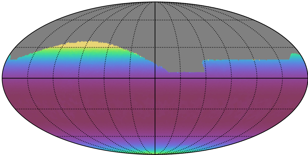
too_100_1v3.4_10yrs All sky r band: Min airmass
