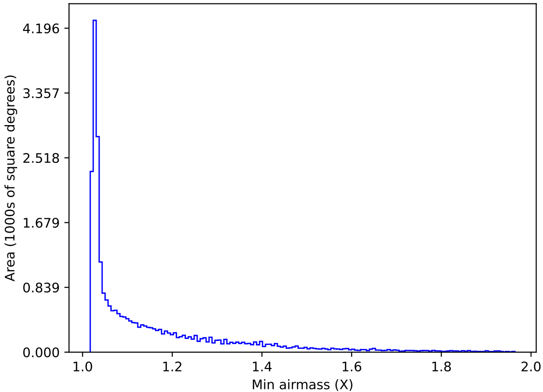
too_100_1v3.4_10yrs All sky r band: Min airmass
