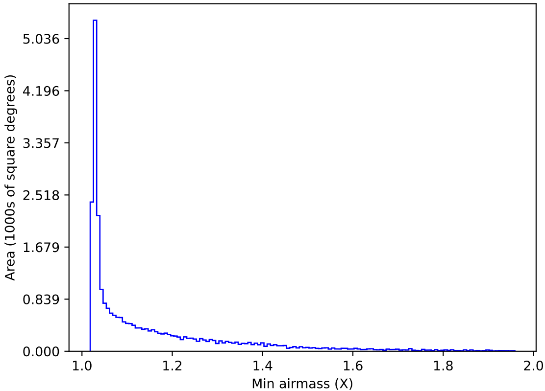
too_100_1v3.4_10yrs All sky i band: Min airmass
