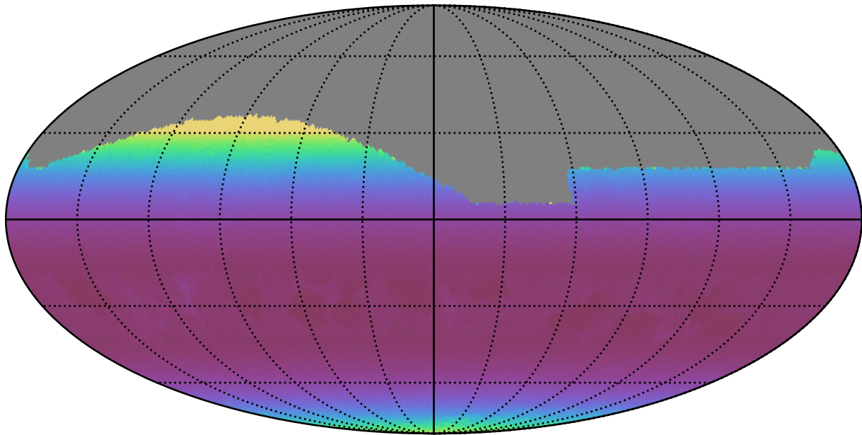
too_100_1v3.4_10yrs All sky g band: Min airmass
