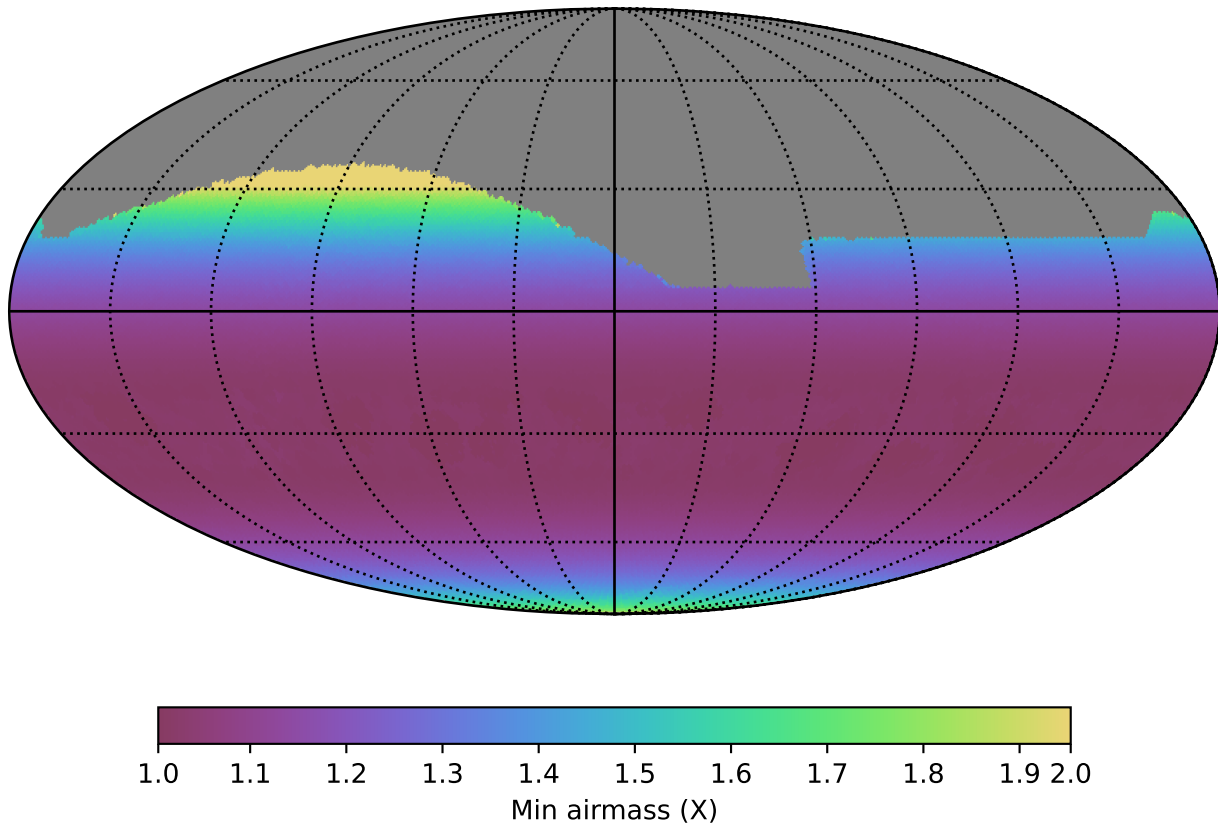
too_100_1v3.4_10yrs All sky all bands: Min airmass
