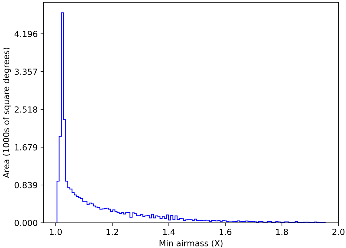
too_100_1v3.4_10yrs All sky all bands: Min airmass
