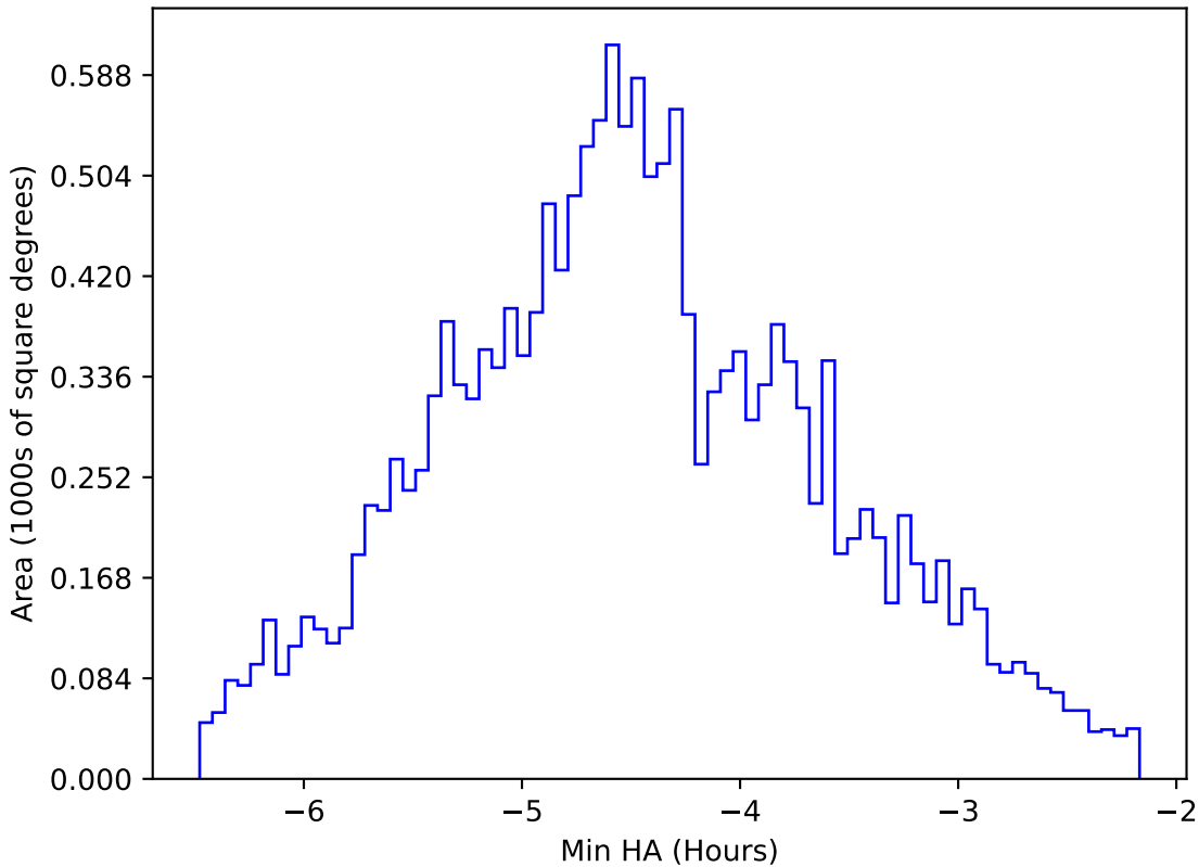
too_100_1v3.4_10yrs WFD z band: Min HA
