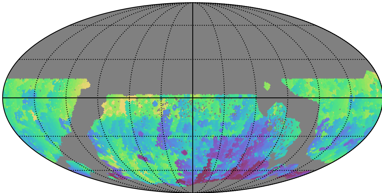
too_100_1v3.4_10yrs WFD u band: Min HA
