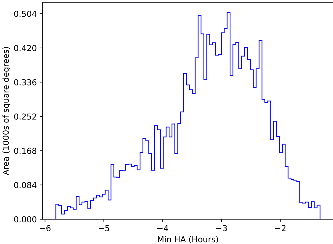
too_100_1v3.4_10yrs WFD u band: Min HA
