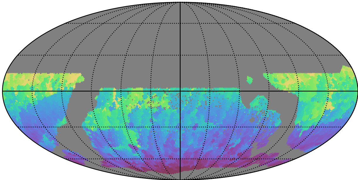
too_100_1v3.4_10yrs WFD i band: Min HA
