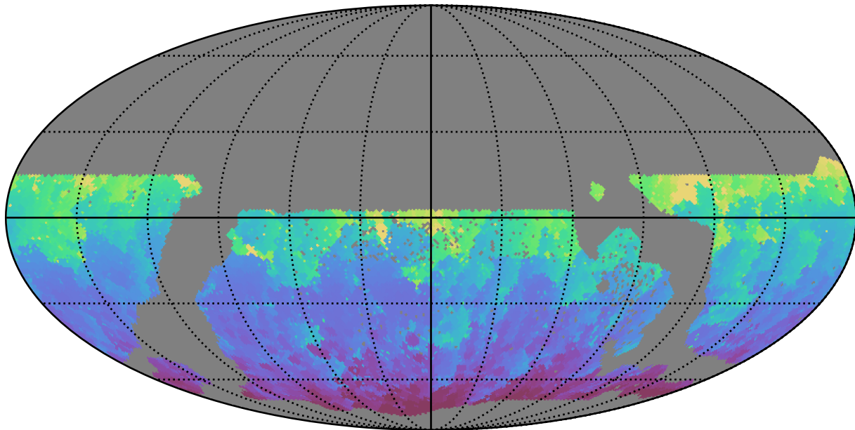
too_100_1v3.4_10yrs WFD g band: Min HA
