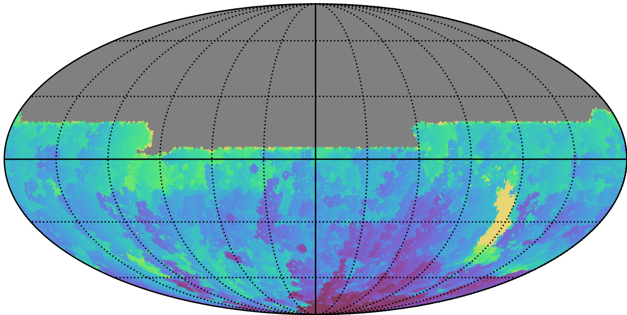
too_100_1v3.4_10yrs All sky u band: Min HA
