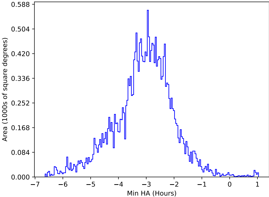
too_100_1v3.4_10yrs All sky u band: Min HA
