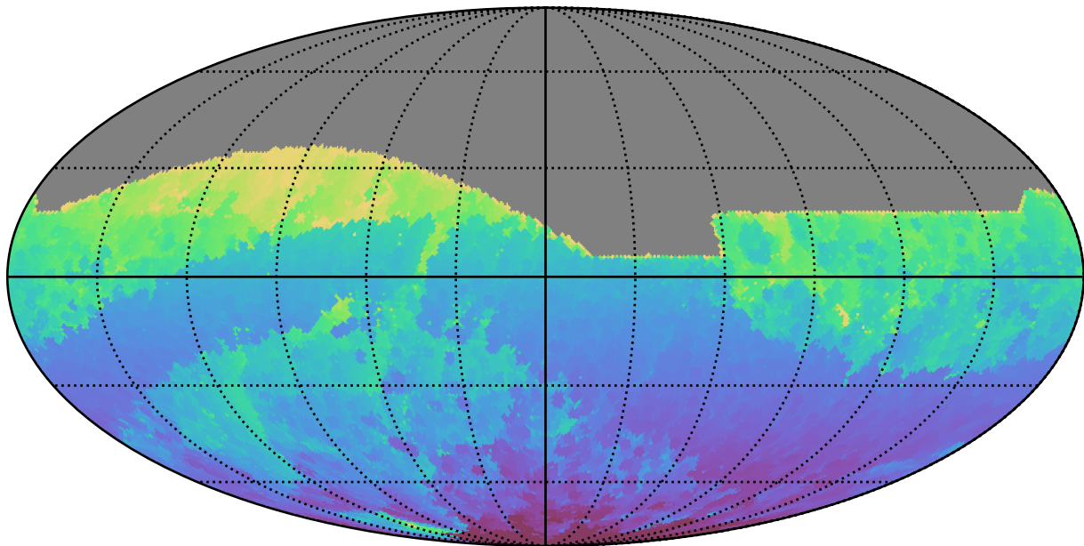
too_100_1v3.4_10yrs All sky r band: Min HA
