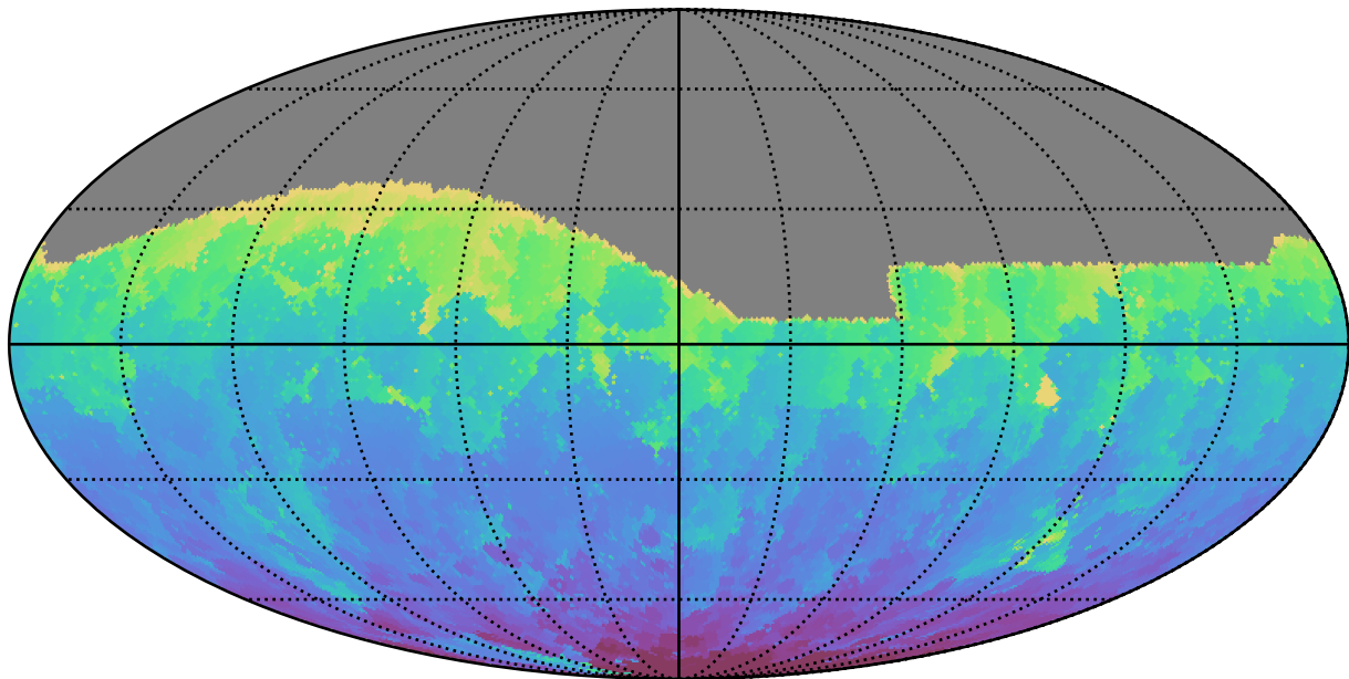
too_100_1v3.4_10yrs All sky g band: Min HA
