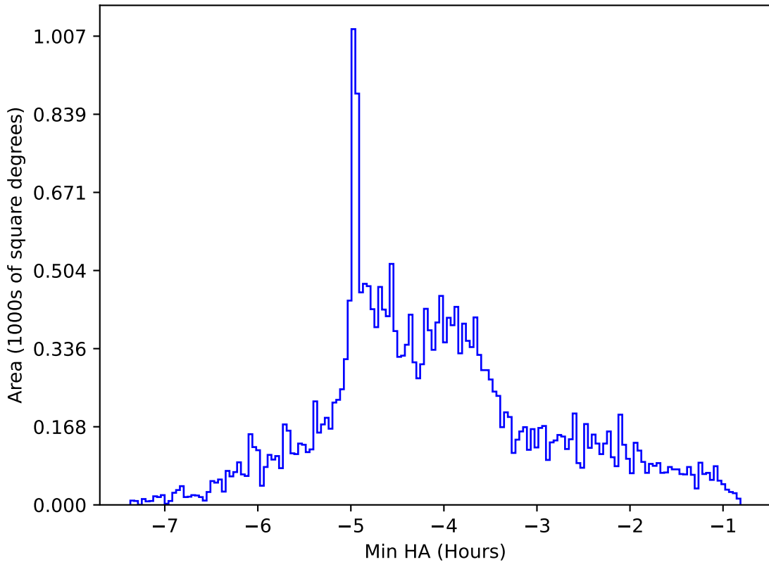
too_100_1v3.4_10yrs All sky g band: Min HA
