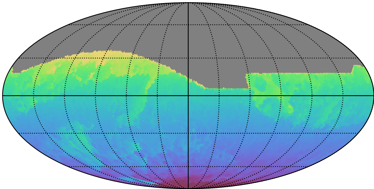
too_100_1v3.4_10yrs All sky all bands: Min HA
