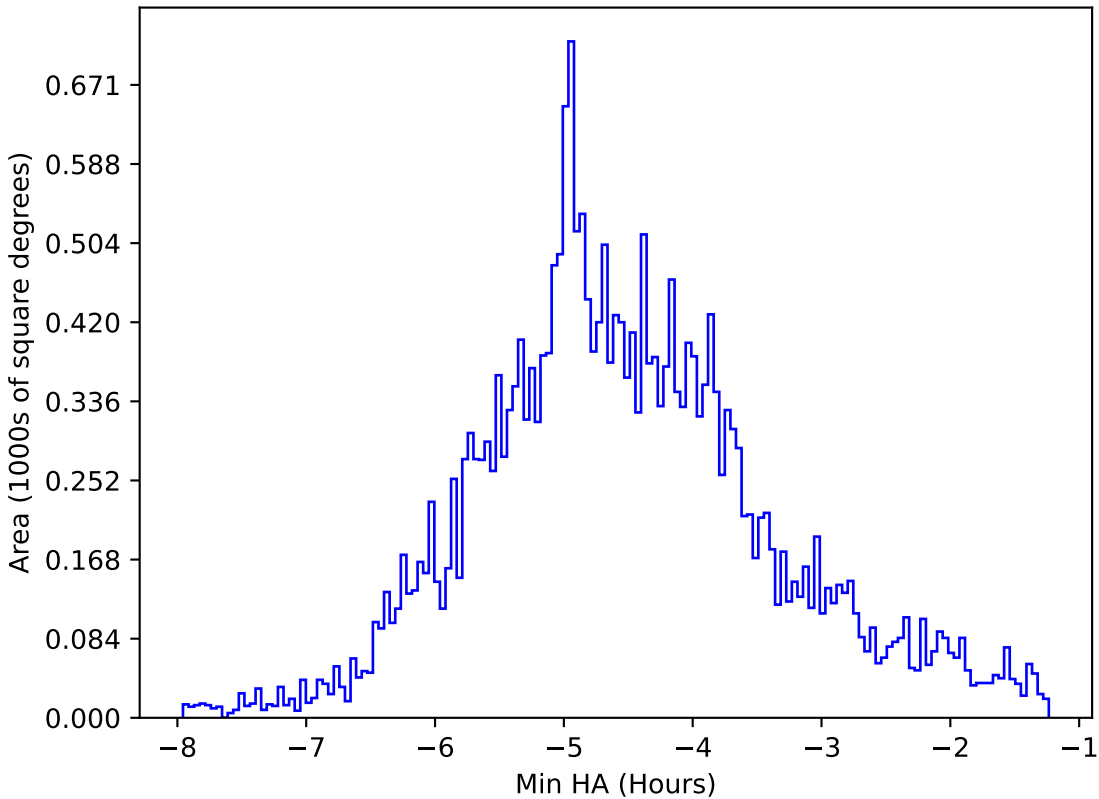
too_100_1v3.4_10yrs All sky all bands: Min HA
