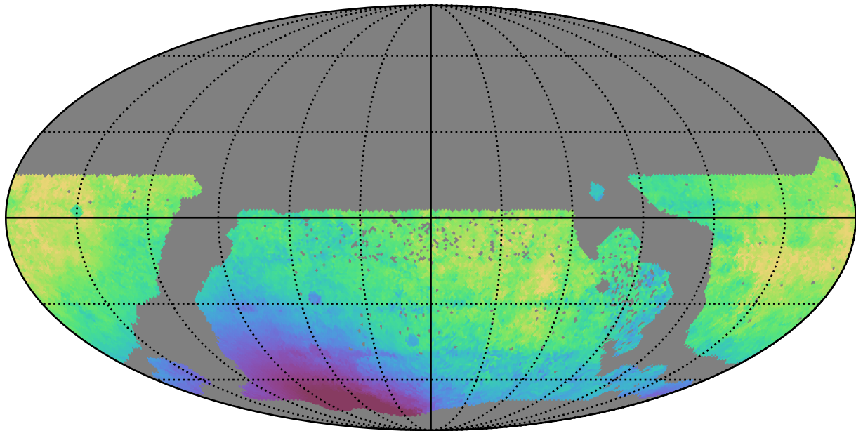
too_100_1v3.4_10yrs WFD z band: Median solarElong
