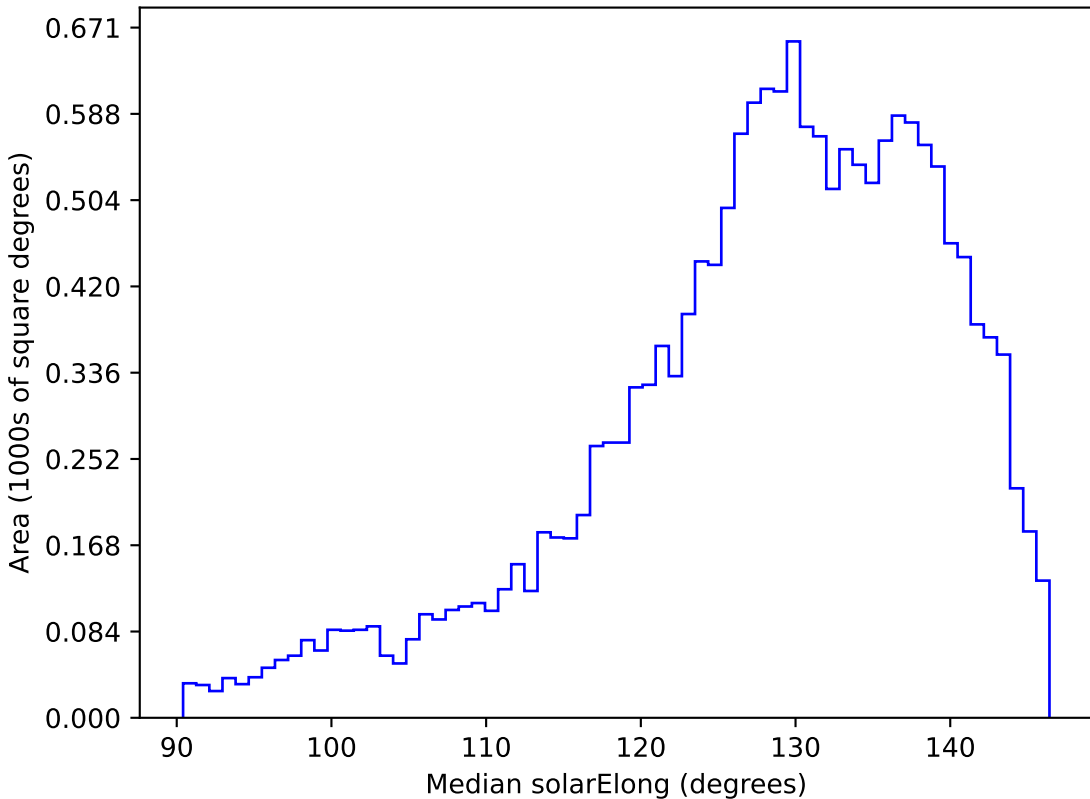
too_100_1v3.4_10yrs WFD z band: Median solarElong
