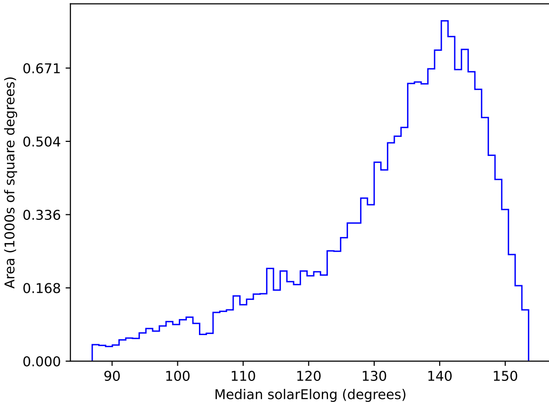
too_100_1v3.4_10yrs WFD u band: Median solarElong
